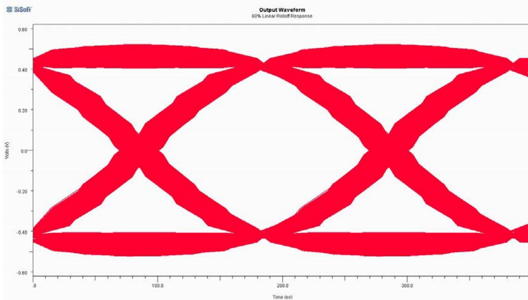
Figure 4: Eye diagram for a 60% linear rolloff response
