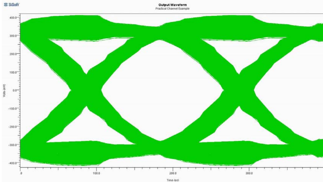
Figure 3: Eye diagram for a practical channel
