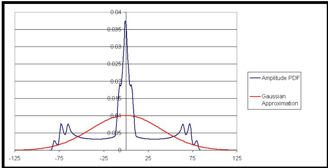
Figure 9: Amplitude PDF for a plesiochronous 60% linear rolloff aggressor
