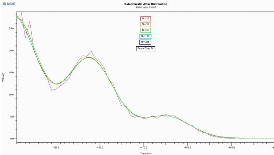
Figure 5: Deterministic Jitter PDF for 60% linear rolloff pulse response
