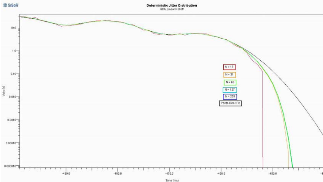
Figure 6: Log scale plot of Deterministic Jitter PDF for 60% linear rolloff pulse response
