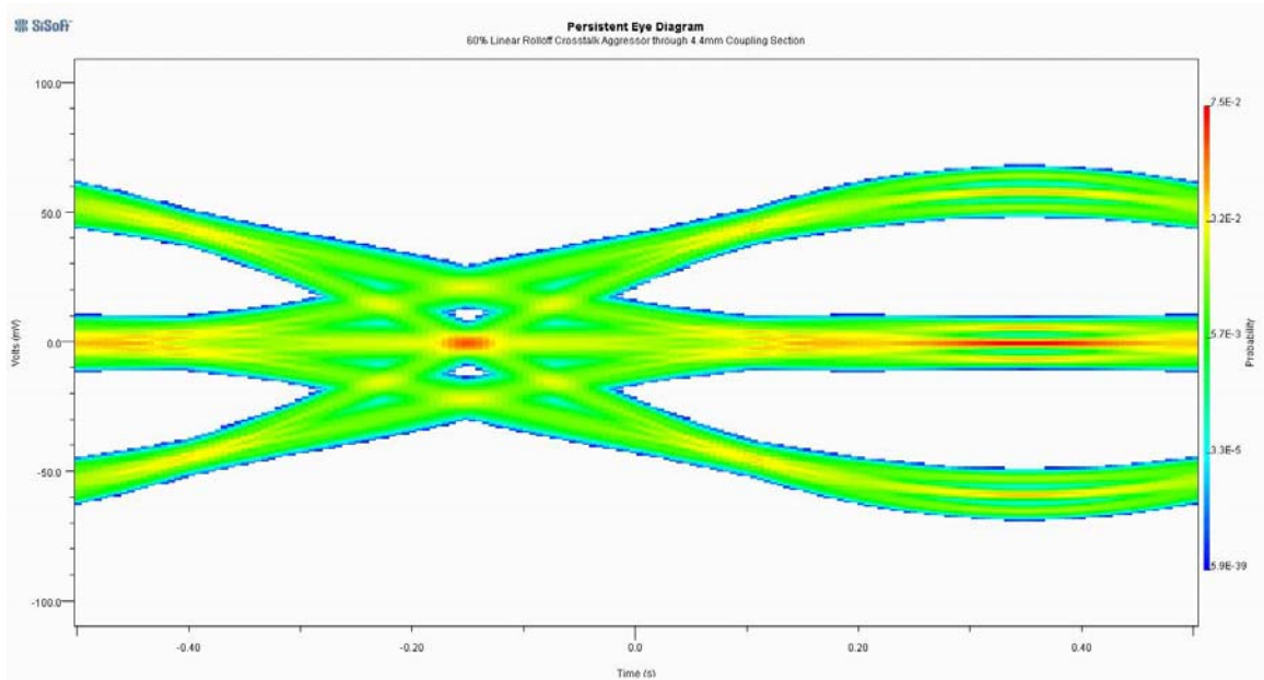
Figure 8: Crosstalk coupled eye for 60% linear rolloff response
