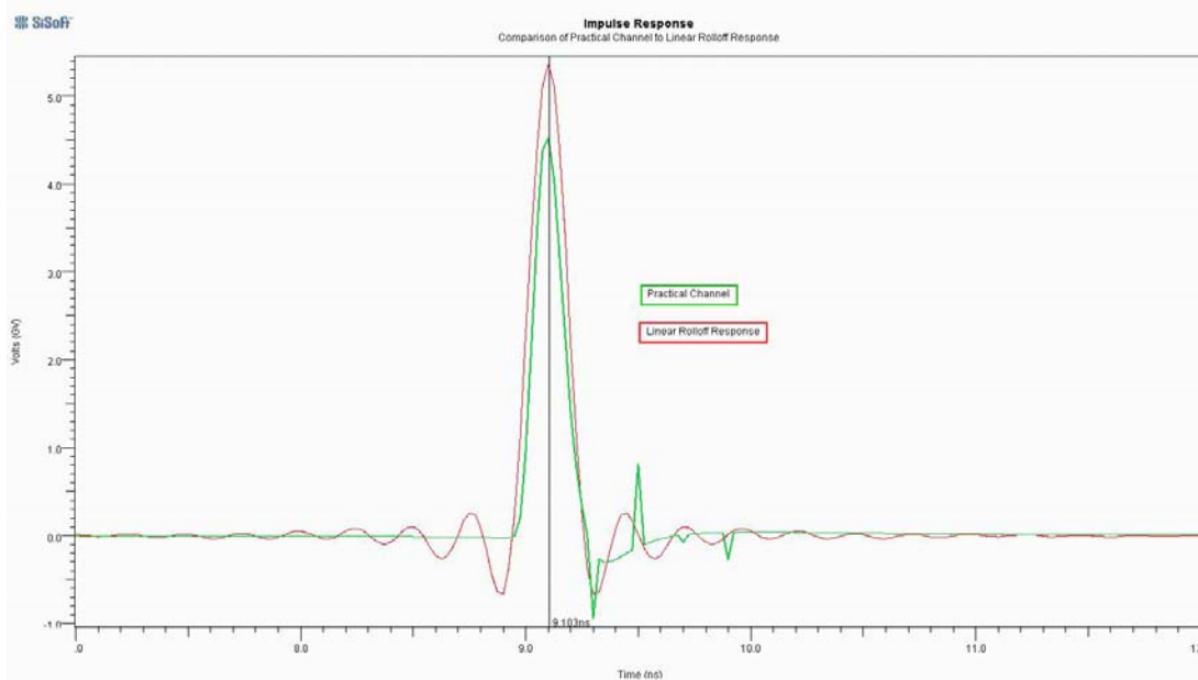
Figure 2: Impulse response comparison between practical channel and a 60% linear rolloff pulse shape
